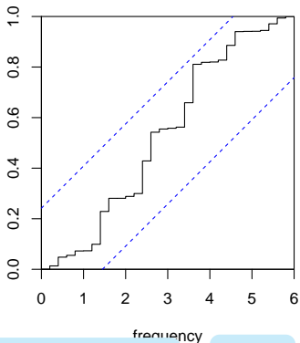
Series: resid(snaive(ldeaths))
