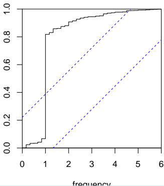
Series: Ideaths
